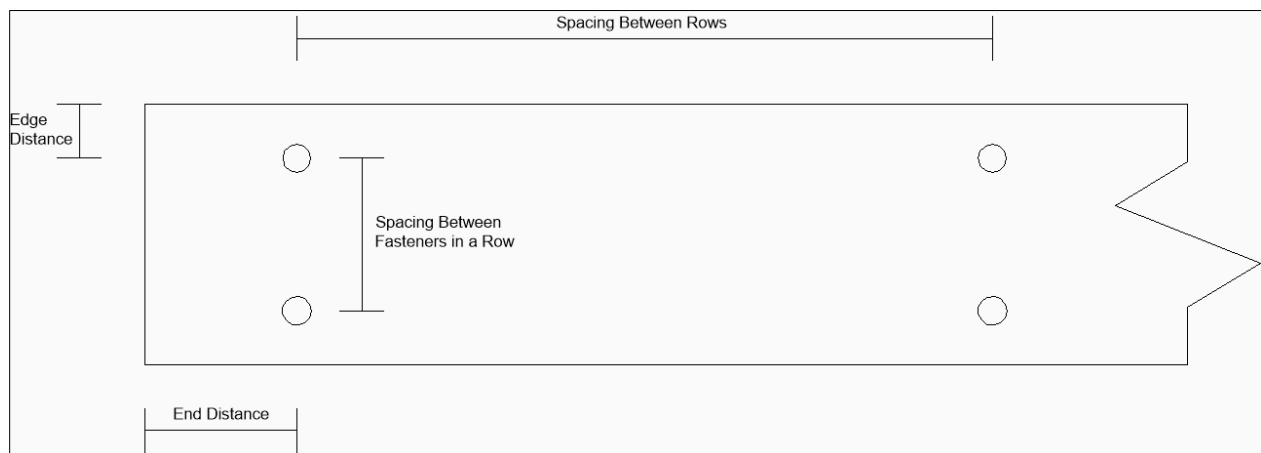
Figure 9. Minimum Screw Spacing Reference
